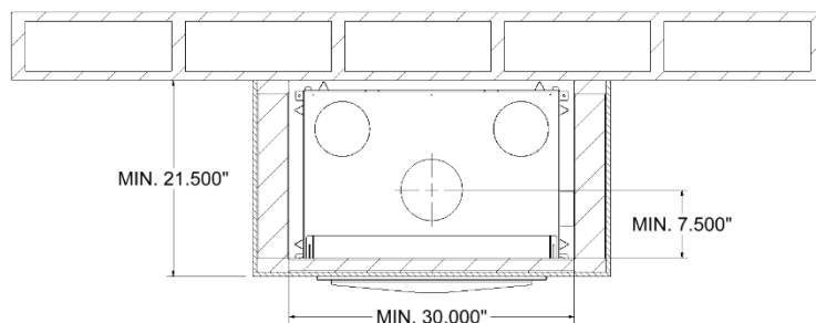
Illustration 3-2: Installation mur droit
