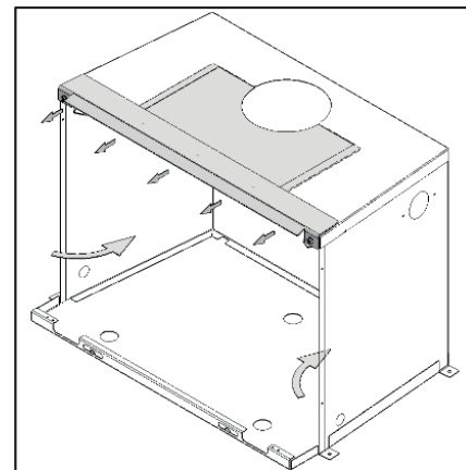
Illustration 2-11: Chambre de circulation
